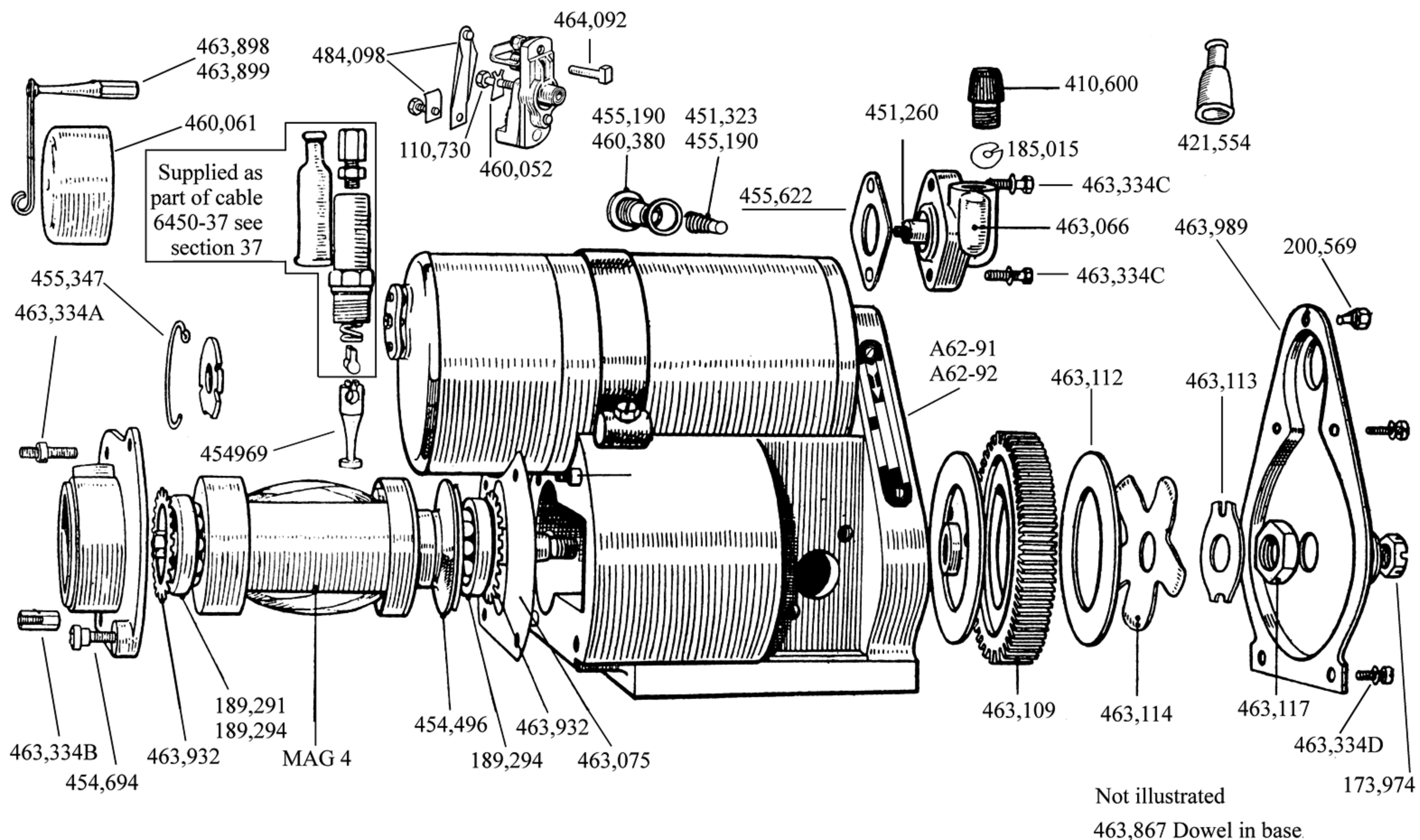
MO Series Magneto as fitted to BSA Singles
